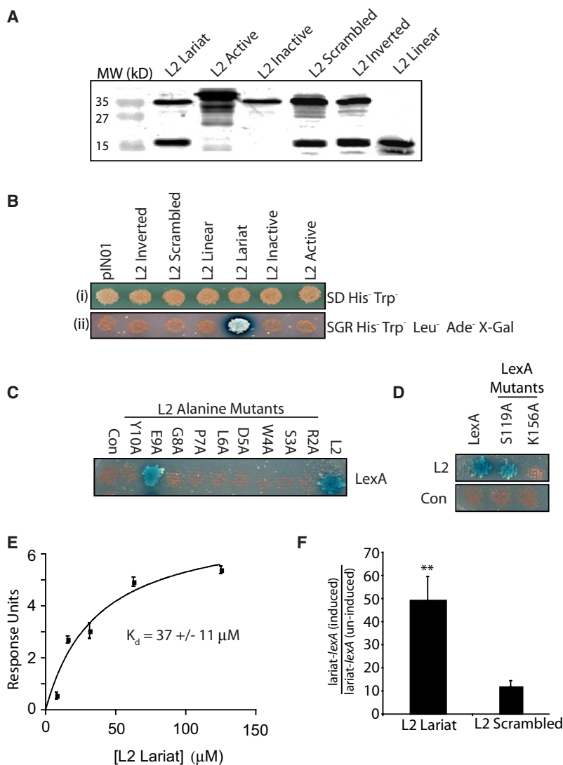
Figure 3. Analysis of the L2 Lariat
