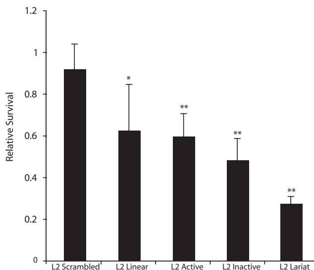
Figure 6. Survival Assay for MMC-Treated BL21-CP Cells Transformed with L2 Lariat and Intein Constructs
