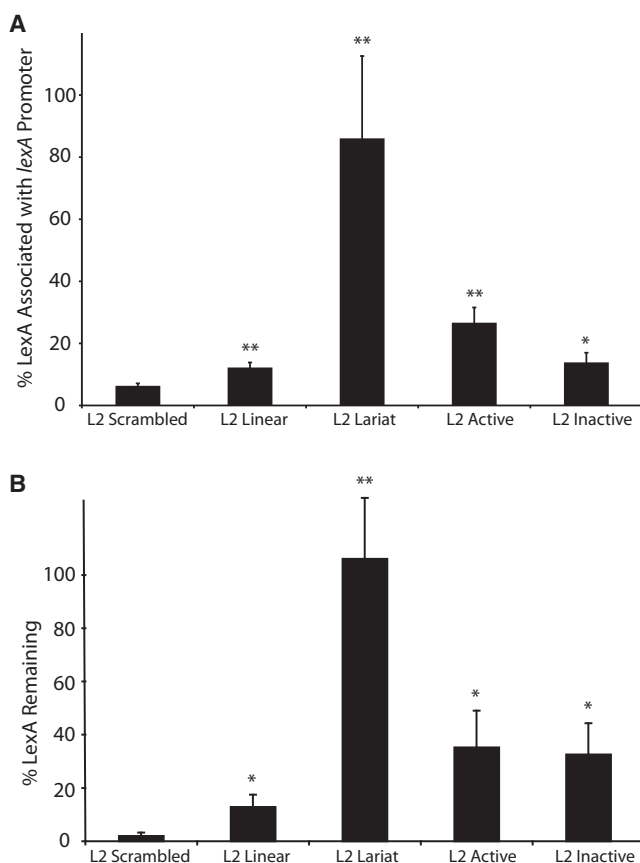
Figure 5. L2 Lariat Inhibition of LexA Autoproteolysis
