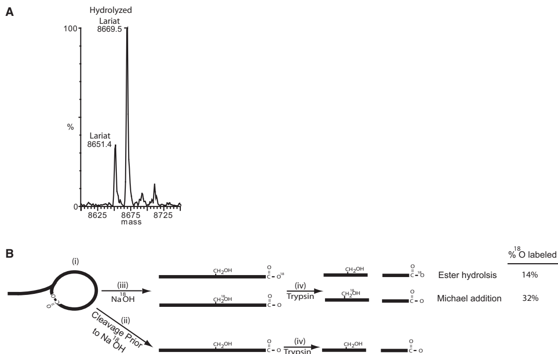
Figure 4. Stability of L2 Lariat
