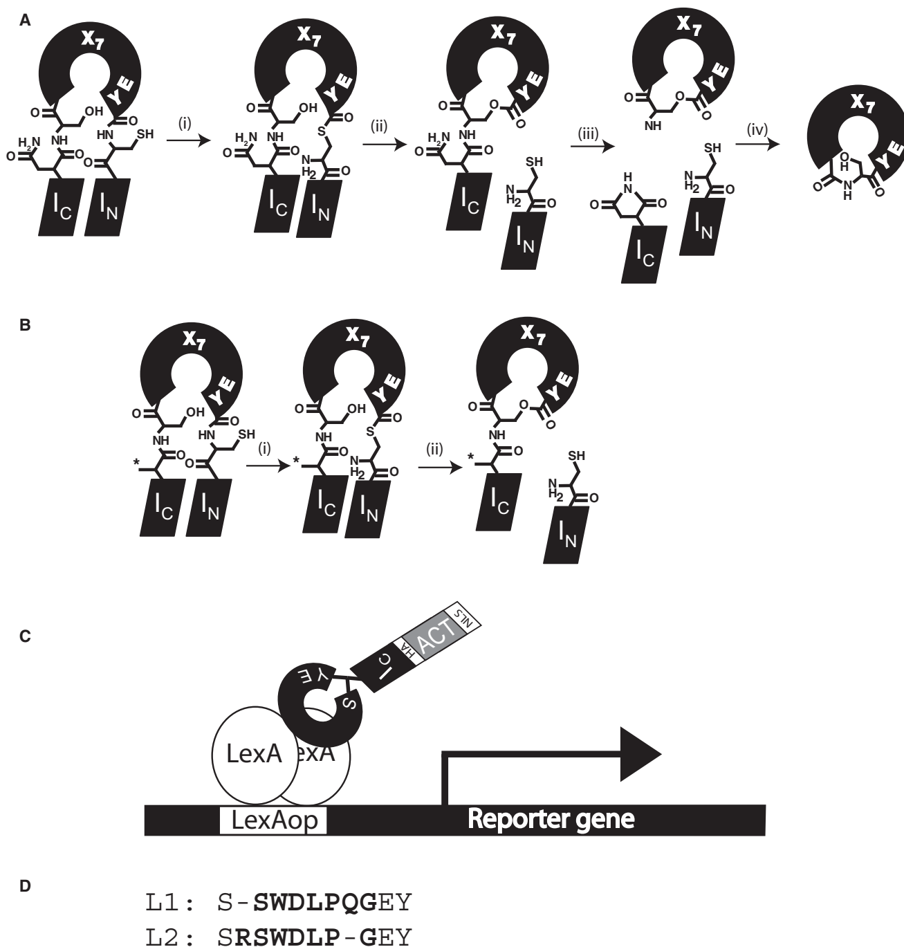
Figure 1. Production and Isolation of Anti-LexA Lariats
